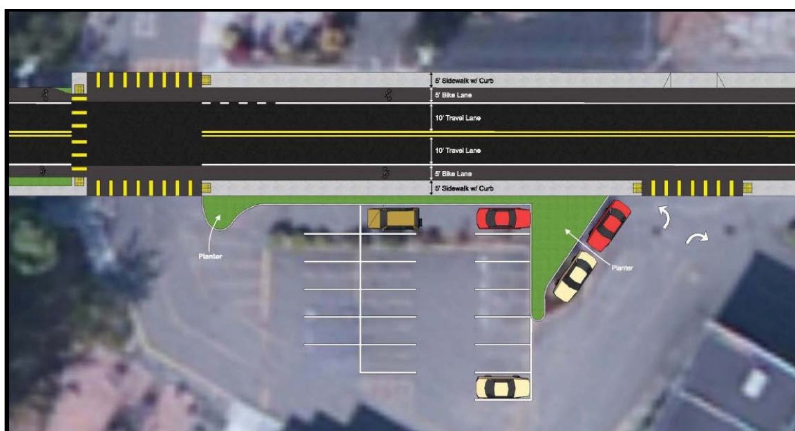
Figure 3.5 Proposed cross-section of the Jacoby Creek School Frontage with the proposed sidewalk option stated in Alternatives Three and Four (SHN et al., 2017).
