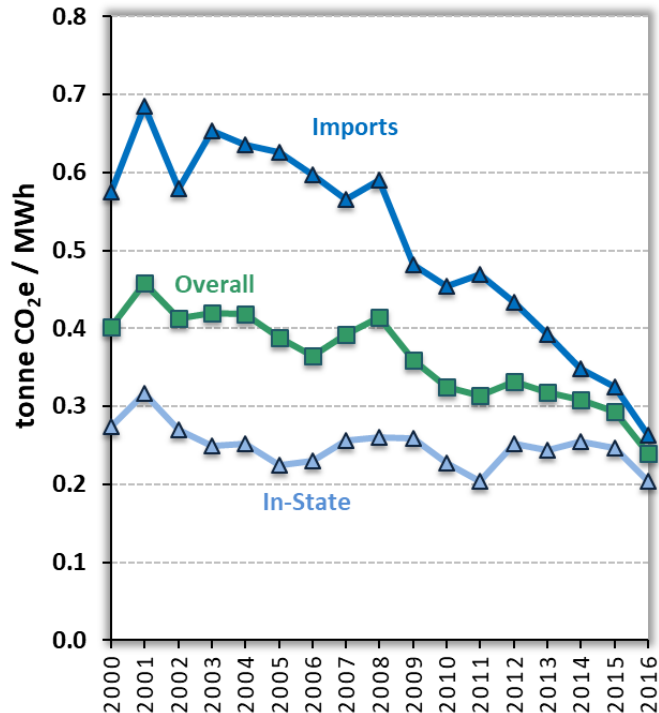
Figure 8. GHG Intensity of Electricity Generation.* This figure shows trends in GHG intensities of electricity generated by in-state power plants, electricity imported from outside of California, and the overall GHG intensities aggregating both in-state generation and electricity imports.
